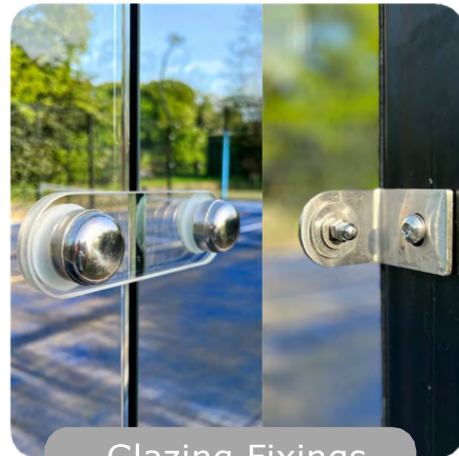
Glazing Fixings
